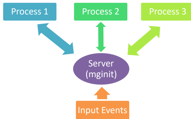
Figure 4.6 Communication mechanism of MiniGUI-Processes runtime mode
